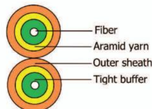
Indoor Duplex Cable
