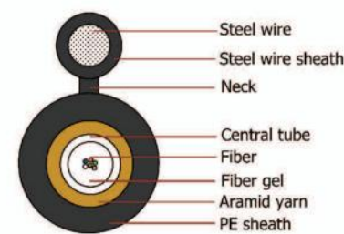
GYXTC8S Cable
